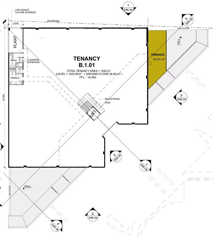
2 FIRST FLOOR PLAN SCALE 1:200
