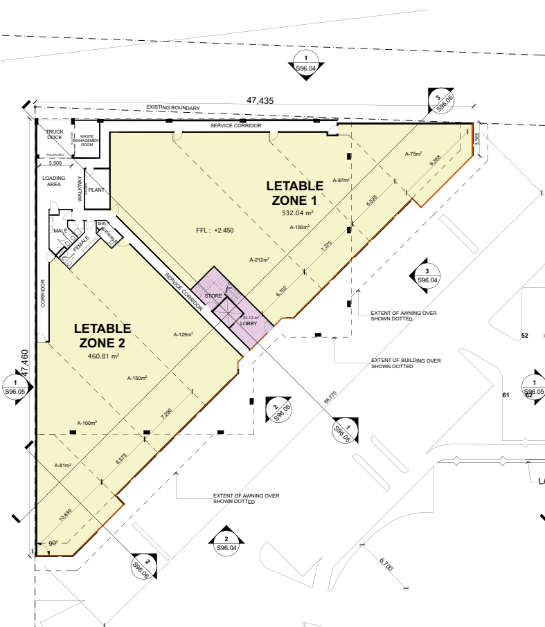
1 GROUND FLOOR PLAN SCALE 1:200
