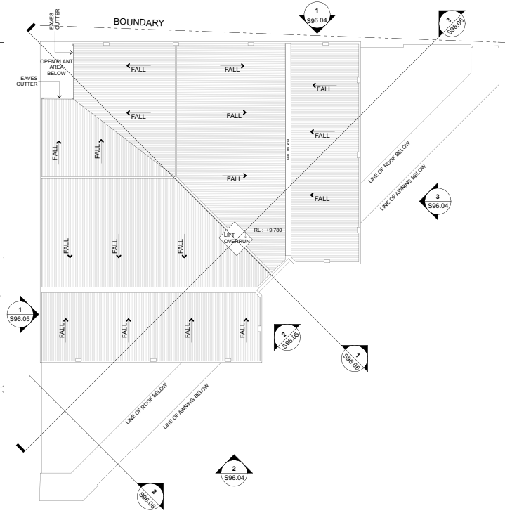
3 ROOF PLAN SCALE 1:200
